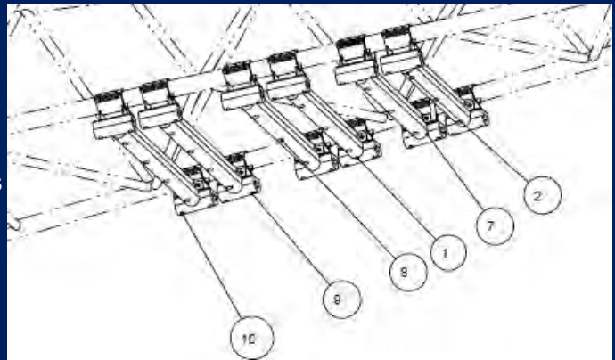
Fig 1. Bumper Bar set on 6/10K Crane
