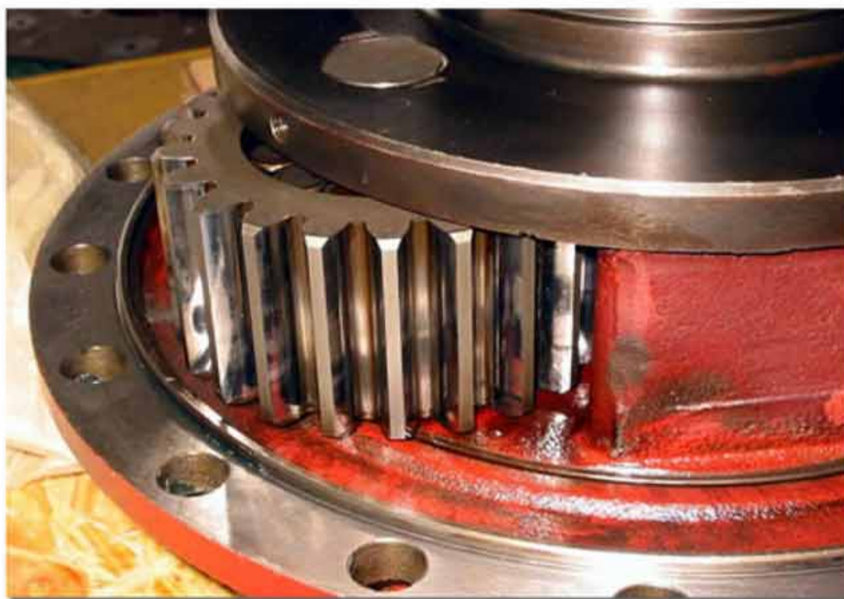
Winch stripdown and rebuilding
